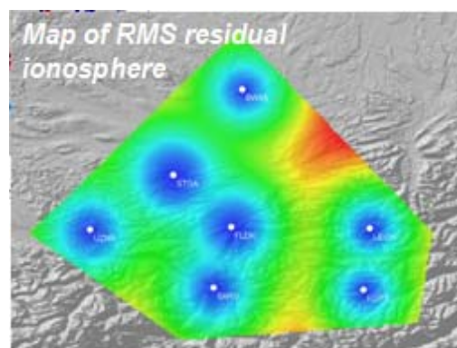
Figure 3: Leica SpiderQC - Example of mapped residual ionosphere
