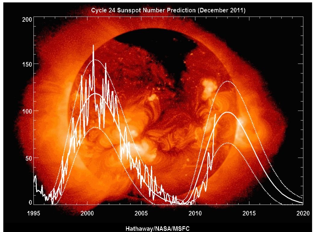
Figure 1 - Solar Cycle no. 24
