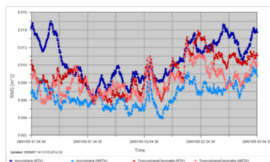
Figure 2 - Leica SpiderQC, Example of Global RMS for Ionosphere & Troposphere, for RTK and NRTK
