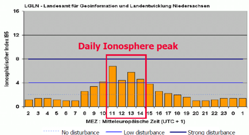
Figure 5 - Ionospheric Index I95
