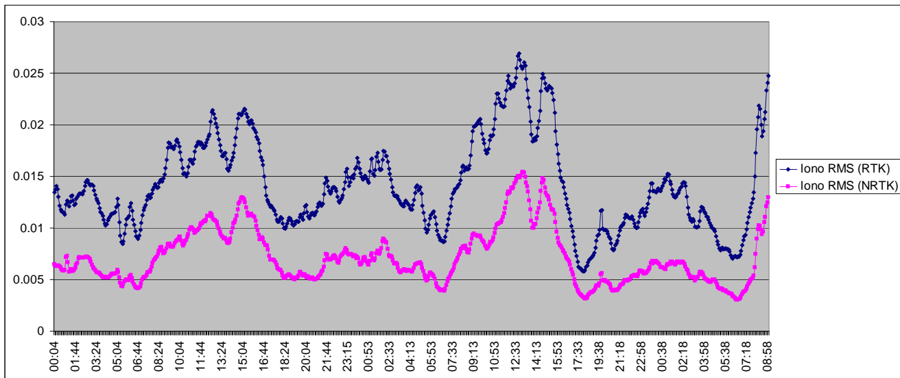
Figure 7 - Ionospheric Residual Variation 17.-19.12.2011
