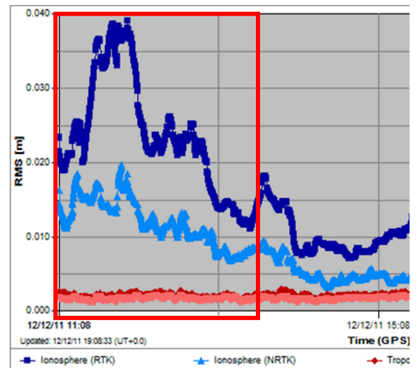
Figure 4 - Leica SpiderQC NOVA Global Ionosphere RMS
