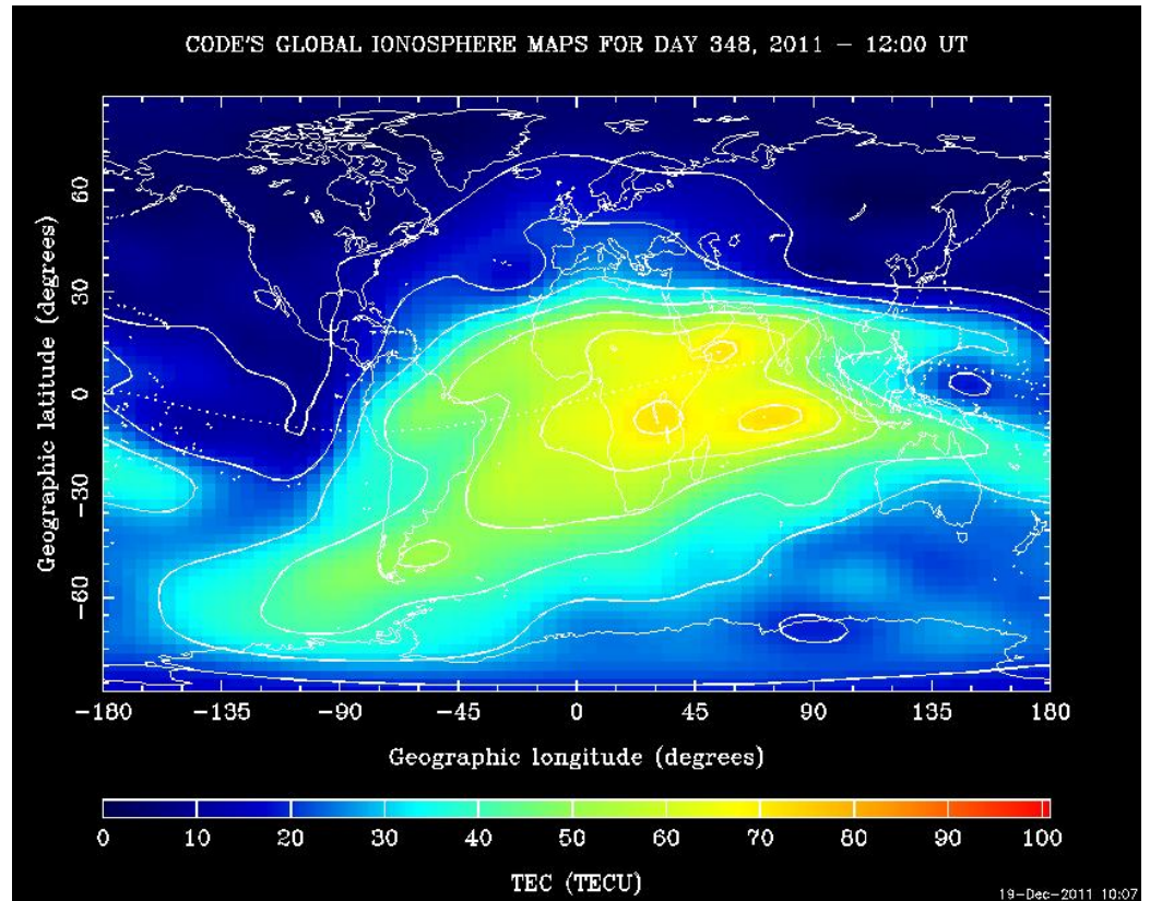
Figure 6 - CODE Global Ionosphere (source: http://aiuws.unibe.ch/ionosphere/gim_12ut.jpg )
